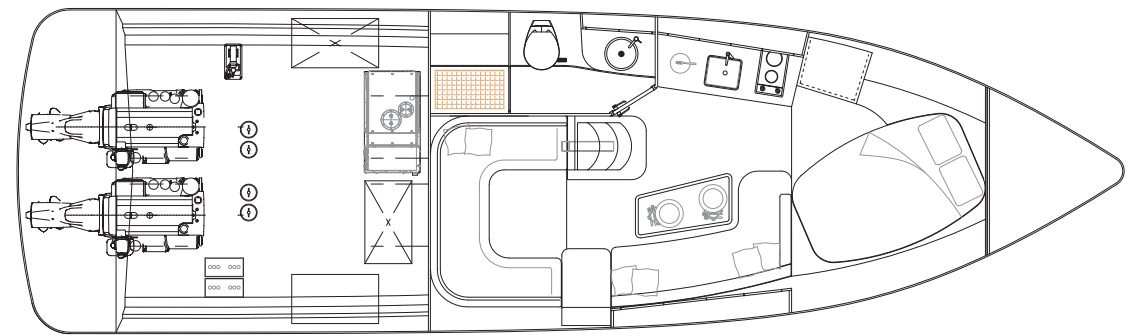
LOWER DECK
